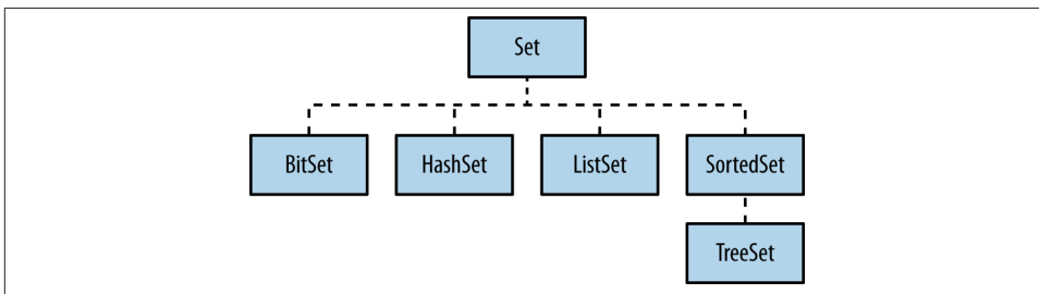
Figure 10-5. Common set classes
